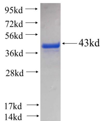
Recombinant human COQ5 SDS-PAGE
