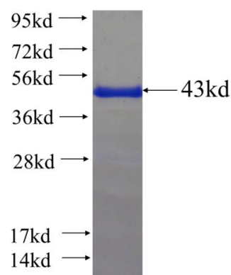
Recombinant human CCDC41 SDS-PAGE
