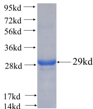
Recombinant human C1orf83(Full length) SDS-PAGE
