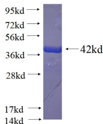
Recombinant human C14orf129 SDS-PAGE
