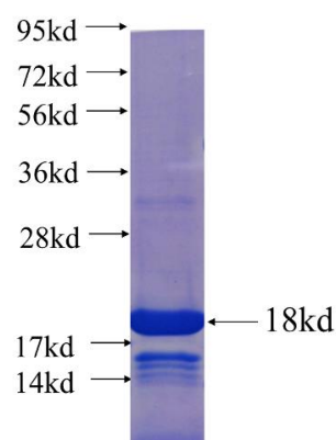
Recombinant human BCAR3 SDS-PAGE
