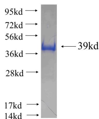
Recombinant human BAG3 SDS-PAGE
