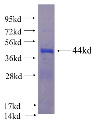
Recombinant human AXL SDS-PAGE
