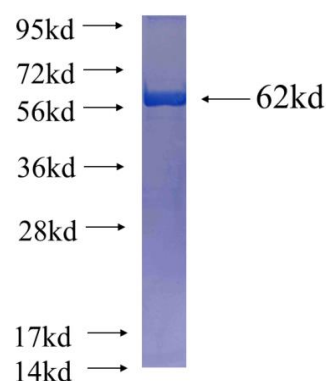
Recombinant human ATP1A1 SDS-PAGE
