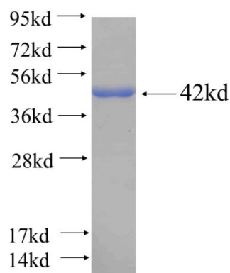
Recombinant human ASNA1(Full length) SDS-PAGE
