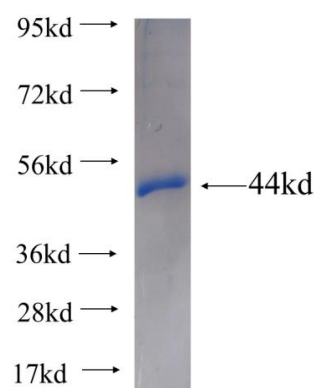
Recombinant human ARIH2 SDS-PAGE
