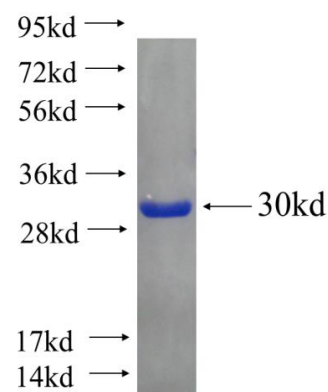
Recombinant human APOL6 SDS-PAGE
