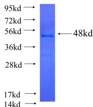
Recombinant human APOBEC4(Full length) SDS-PAGE
