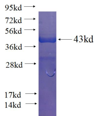
Recombinant human ADIPOR2 SDS-PAGE
