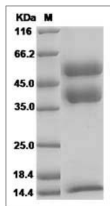
Canine TGF-beta 1 / TGFB1 Protein (His Tag) SDS-PAGE
