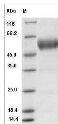
Human SCN3B Protein (Fc Tag) SDS-PAGE
