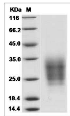
Human SCN2B Protein (His Tag) SDS-PAGE
