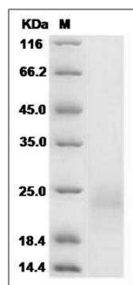
Mouse FAM3D / Oit1 Protein (His Tag) SDS-PAGE
