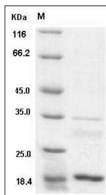
Human UBE2A / HHR6A Protein (His Tag) SDS-PAGE
