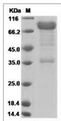
Human RPN2 / Ribophorin II Protein (Fc Tag) SDS-PAGE
