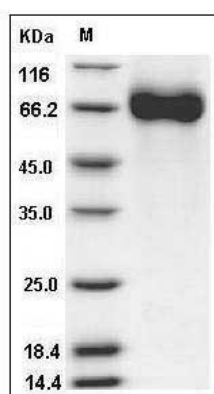
Human CHST15 / GALNAC4S-6ST / BRAG Protein (His Tag) SDS-PAGE
