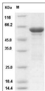
Human ALDOB / Aldolase B Protein GST Tag SDS-PAGE
