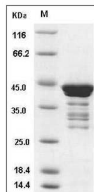
Human C1D Protein (GST Tag) SDS-PAGE
