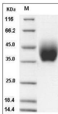
Mouse IL10RB / IL10R2 Protein (His Tag) SDS-PAGE
