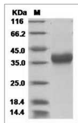
Human HS3ST1 Protein (His Tag) SDS-PAGE
