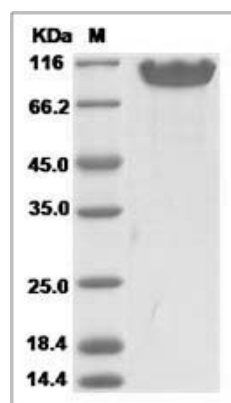
NCAM1 protein SDS-PAGE
