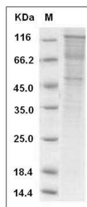
Rat Cadherin-15 / CDH15 Protein (Fc Tag) SDS-PAGE
