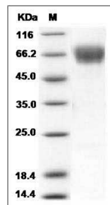
Rat CLEC4F / CLECSF13 Protein SDS-PAGE
