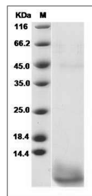
Human CART / CARTPT Protein SDS-PAGE
