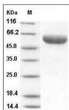
Mouse IL6RA / CD126 Protein (His Tag) SDS-PAGE
