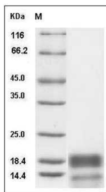
Human GNG13 Protein (His Tag) SDS-PAGE
