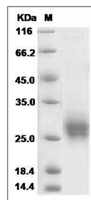
Rat CD90 / THY-1 Protein (His Tag) SDS-PAGE
