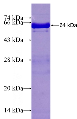
Recombinant Human ZNF326 SDS-PAGE
