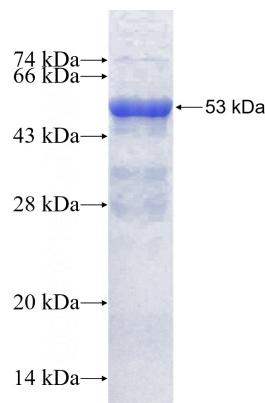
Recombinant Human EIF6 SDS-PAGE
