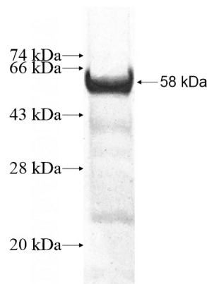
Recombinant Human ZBTB6 SDS-PAGE
