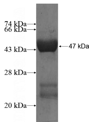
Recombinant Human HINT2 SDS-PAGE
