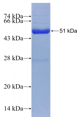
Recombinant Human PSMB6 SDS-PAGE
