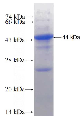
Recombinant Human EXOSC10 SDS-PAGE
