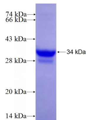
Recombinant Human APOF SDS-PAGE
