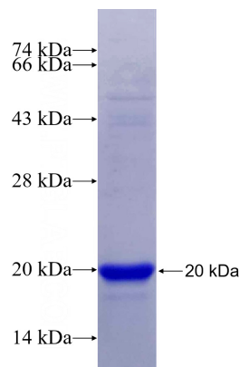
Recombinant Human VASH2 SDS-PAGE
