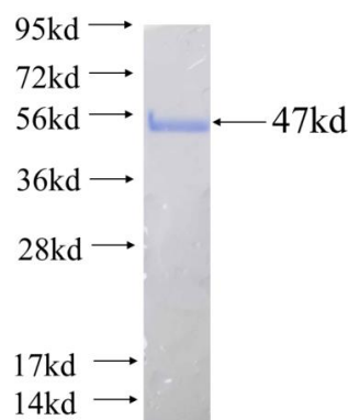
Recombinant Arabidopsis thaliana PDF1A SDS-PAGE
