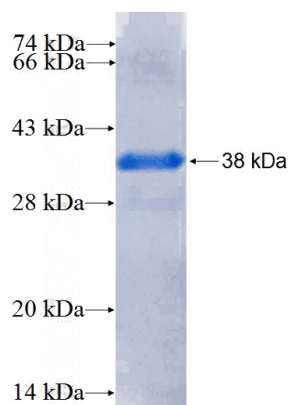
Recombinant Human CYP21A2 SDS-PAGE
