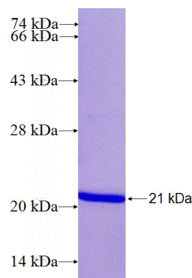
Recombinant Human PSMD8 SDS-PAGE
