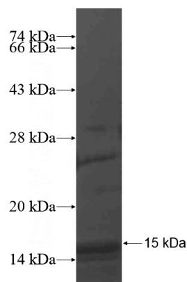
Recombinant Human SLC16A6 SDS-PAGE
