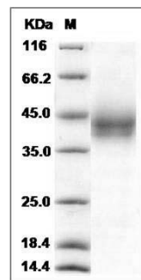
Rat B7-H3 / CD276 Protein (His Tag) SDS-PAGE
