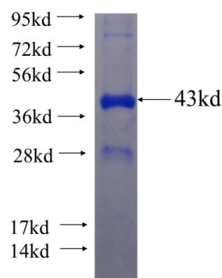
Recombinant human MGAT1 SDS-PAGE
