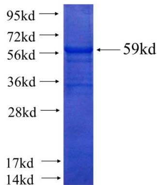
Recombinant human SNX17 SDS-PAGE
