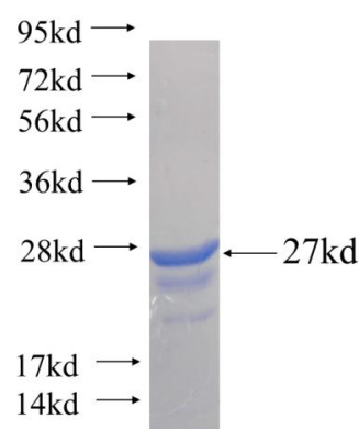
Recombinant human KCNN3 SDS-PAGE
