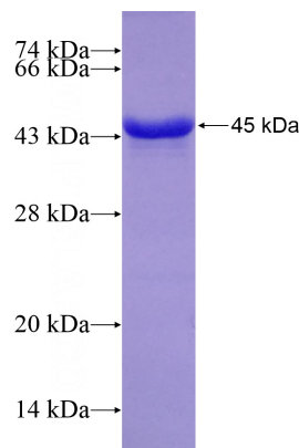
Recombinant Human DCPS SDS-PAGE
