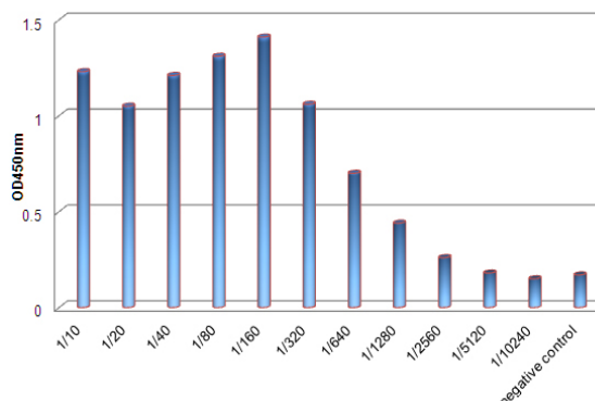
sELISA detection of commercial EGF drug by different dilution.
