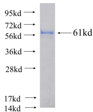
Recombinant human PURA SDS-PAGE
